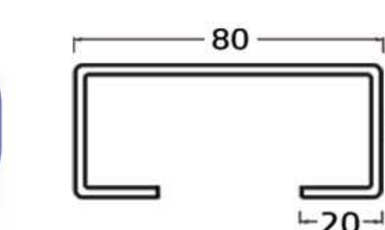
Low Duty Upright
