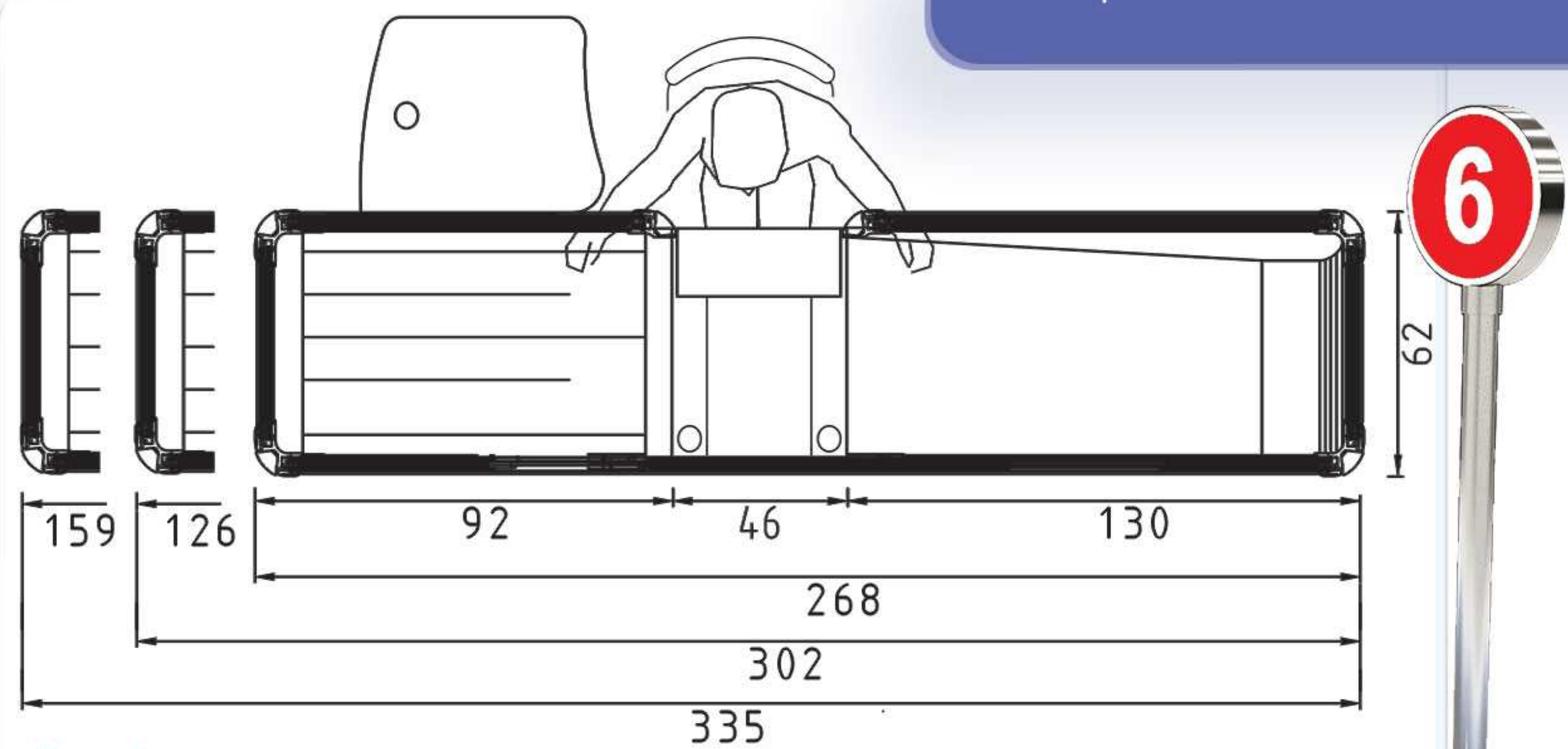
6- Unique Check-out Counter Model I-series
