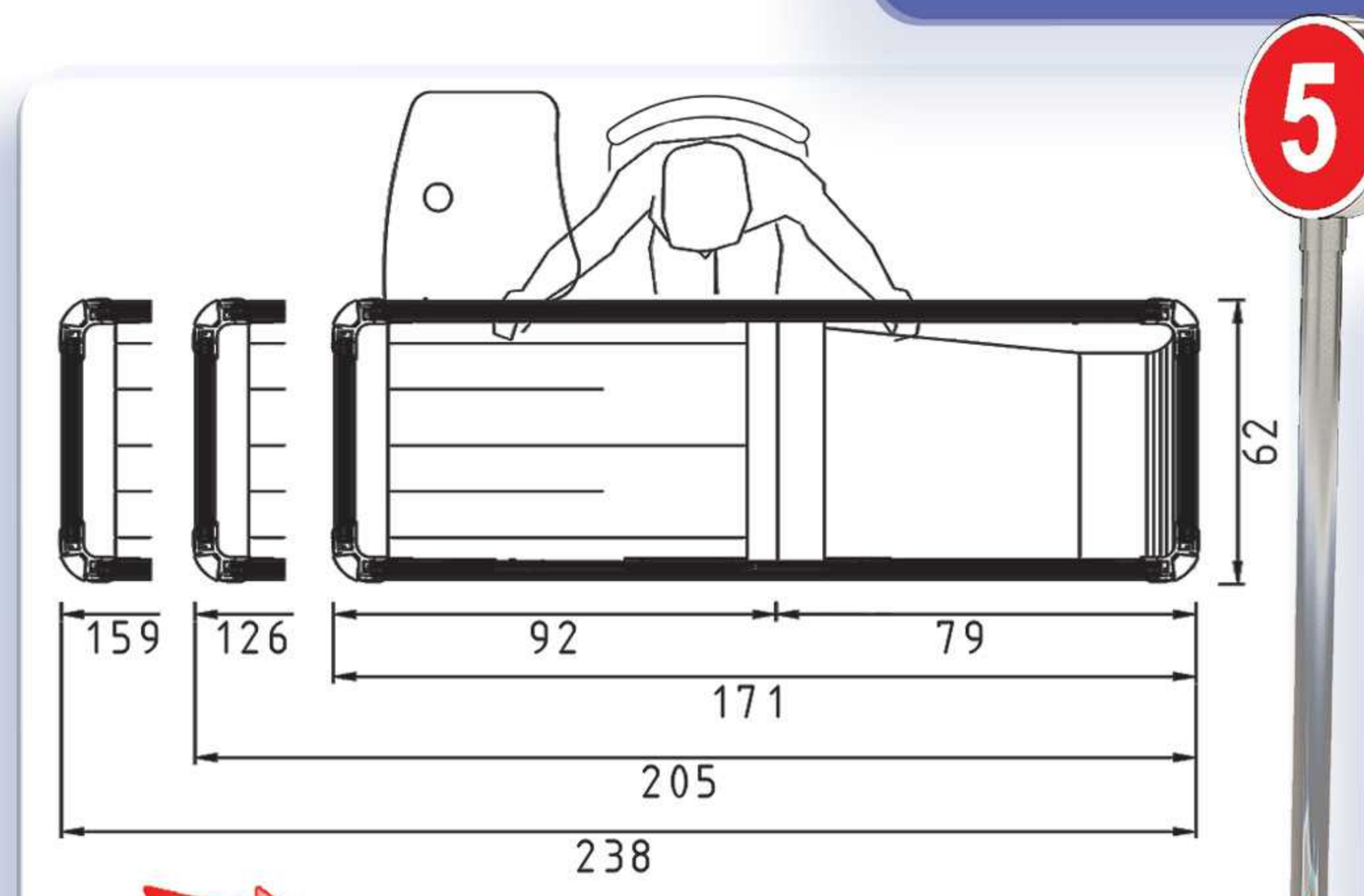
5- Unique Check-out Counter Model I-series
