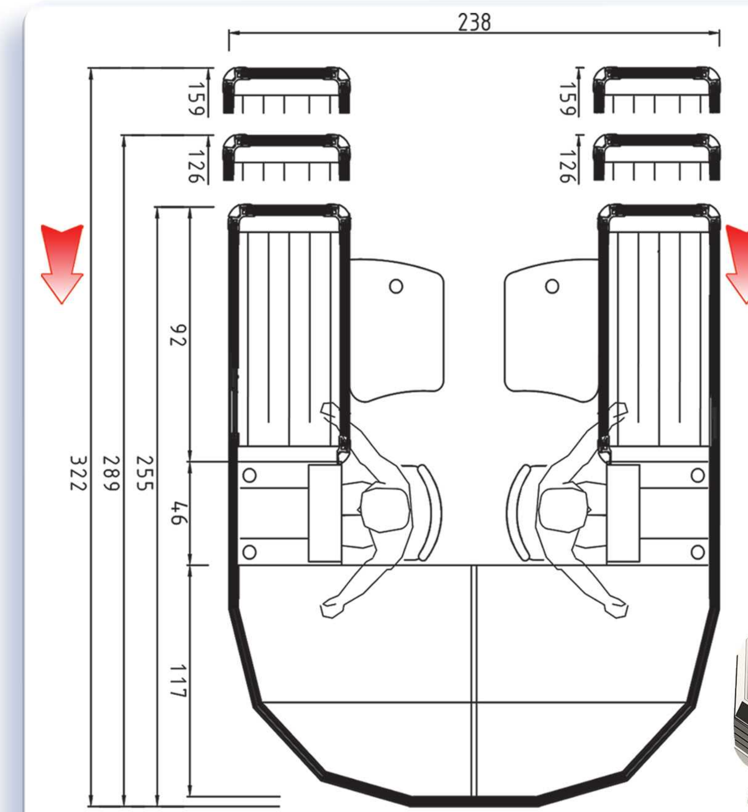
13- Twin Check-out Counter Model U-series
