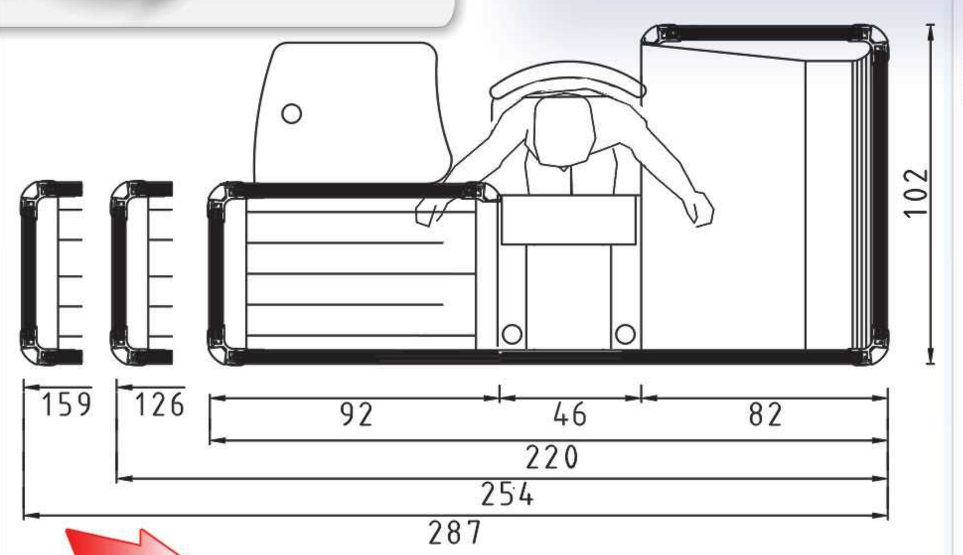
8- Unique Check-out Counter Model L-series
